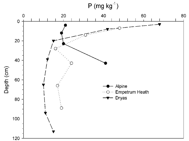
FIGURE 6. Extractable P contents by depth in selected alpine, Empetrum heath , and Dryas soils. Note higher amounts at the surface associate with organic matter except with the alpine soils, where P tends to decrease toward the surface.
